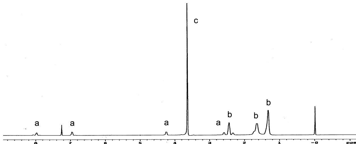
Figure 1. ^1\text{H} NMR spectra of poly(PEG:SA:CPP) (30:50:20) poly(ether–anhydride): a, peaks attributed to CPP; b, peaks attributed to SA; c, peak attributed to PEG.
