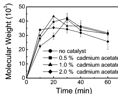
Figure 3. Molecular weight of poly(PEG:SA) (30:70) as a function of reaction time (with catalyst, vacuum \sim 0.08 Torr). Polymers were melt-polymerized at 180^\circ\text{C} in the presence of cadmium acetate ( \text{CdAc}_2 ).
