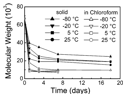
Figure 4. Stability profiles of poly(PEG:SA:CPP) (30:50:20) in the solid state and in anhydrous chloroform at four storage temperatures. Polymerization conditions were 30 min at 180 °C without catalyst.
