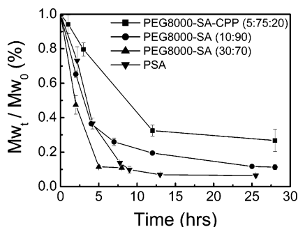
Figure 6. Degradation profiles of poly(ether-anhydride) microspheres in PBS (pH 7.4, 37 °C).
