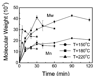
Figure 2. Molecular weight of poly(PEG:SA) (30:70) as a function of reaction time at different temperatures (without catalyst, vacuum \sim 0.08 Torr).
